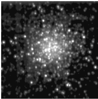
M13 - 4/23/03
