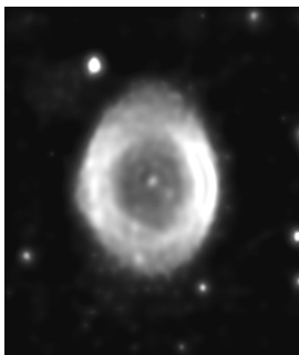
M57 - 4/23/03
