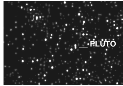
PLUTO - 5/21/03
