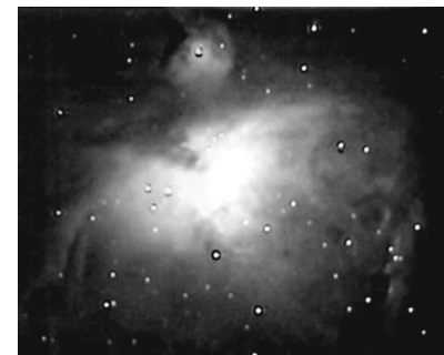
M42 - 3/30/03
