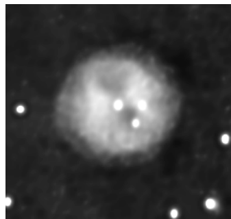
M97 - 4/23/03
