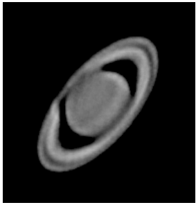
SATURN - 3/30/03
