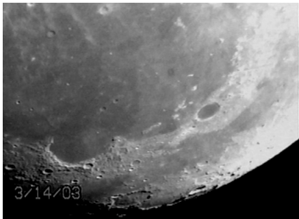
MOON - 3/14/03
