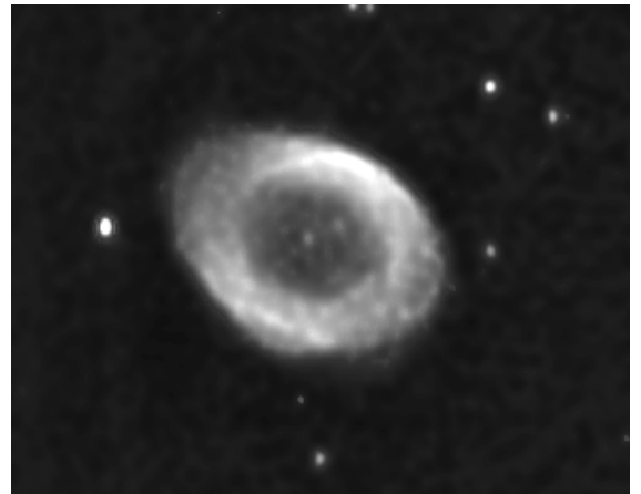
M57 - Ring Nebula
