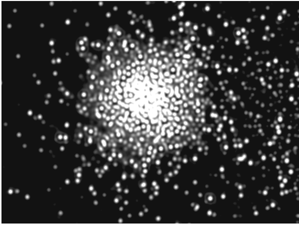
M13 – Hercules Globular Cluster (M13-shot 3)
